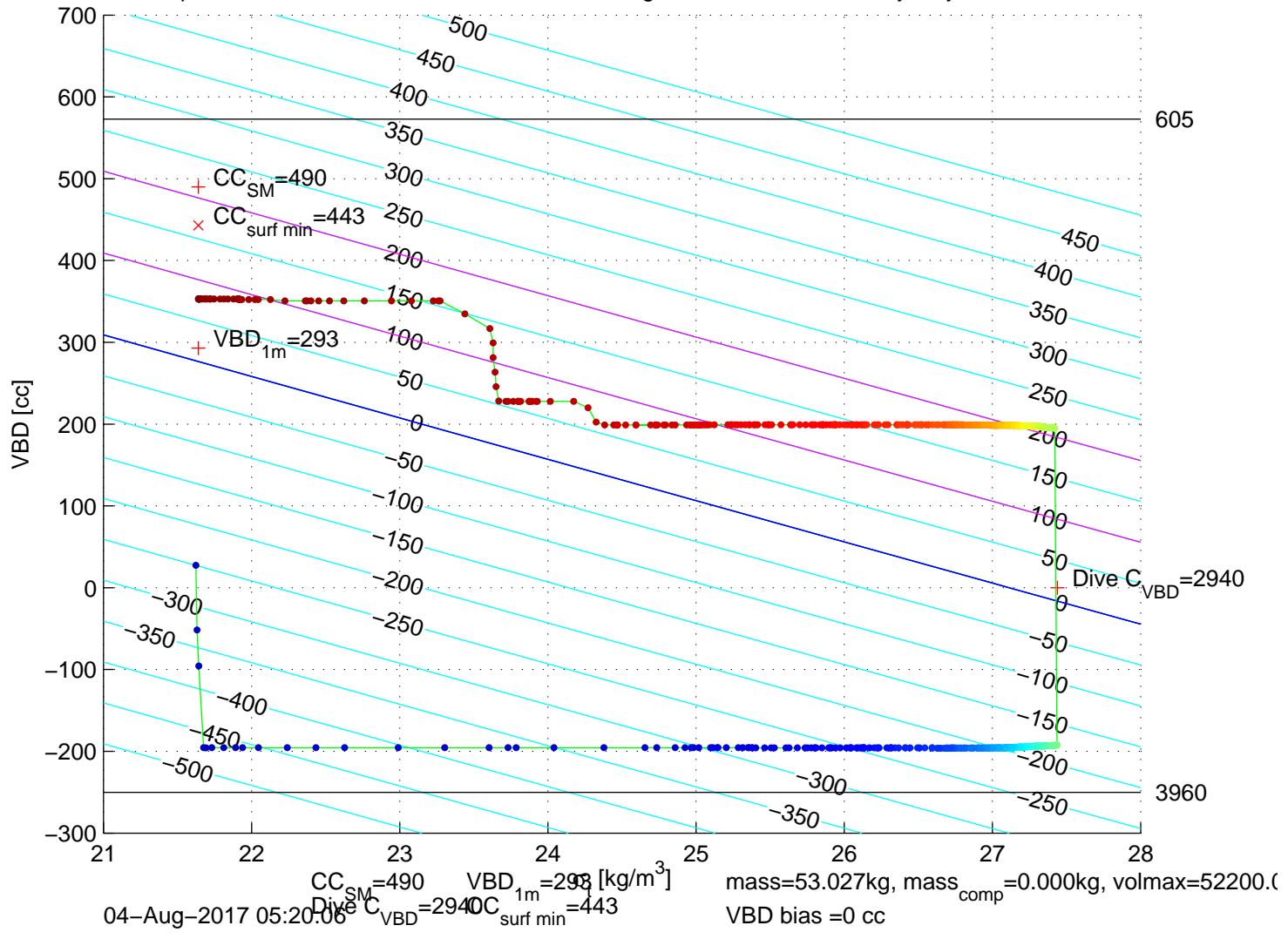
p6300159: SG630 Mission 7 Jul 2017 04-Aug-2017 06:02:31Z – buoyancy contoured
