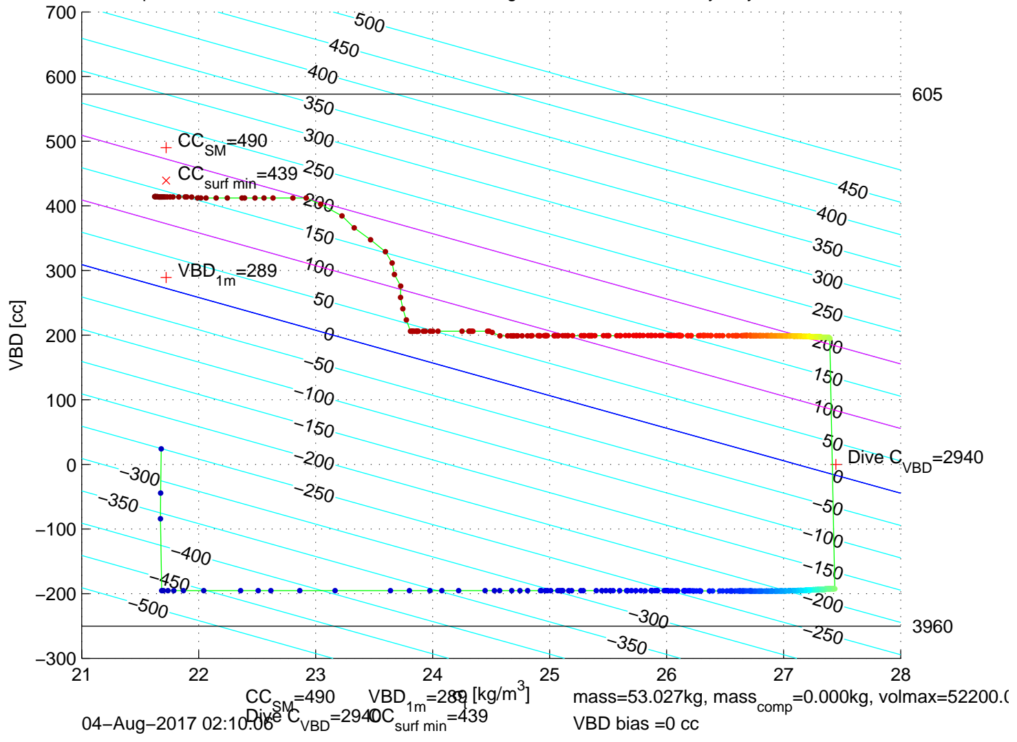
p6300158: SG630 Mission 7 Jul 2017 04–Aug–2017 03:03:40Z – buoyancy contoured
