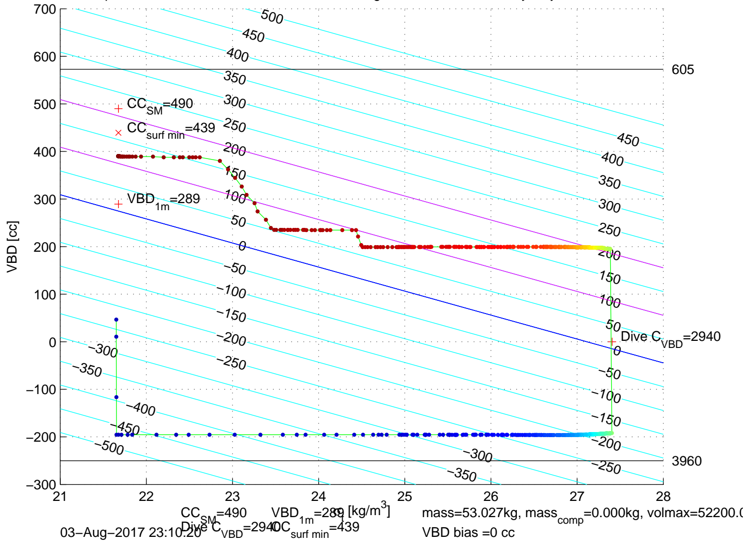
p6300157: SG630 Mission 7 Jul 2017 04-Aug-2017 00:05:22Z – buoyancy contoured
