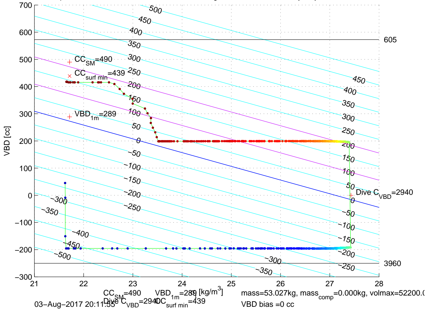
p6300156: SG630 Mission 7 Jul 2017 03-Aug-2017 21:04:27Z - buoyancy contoured
