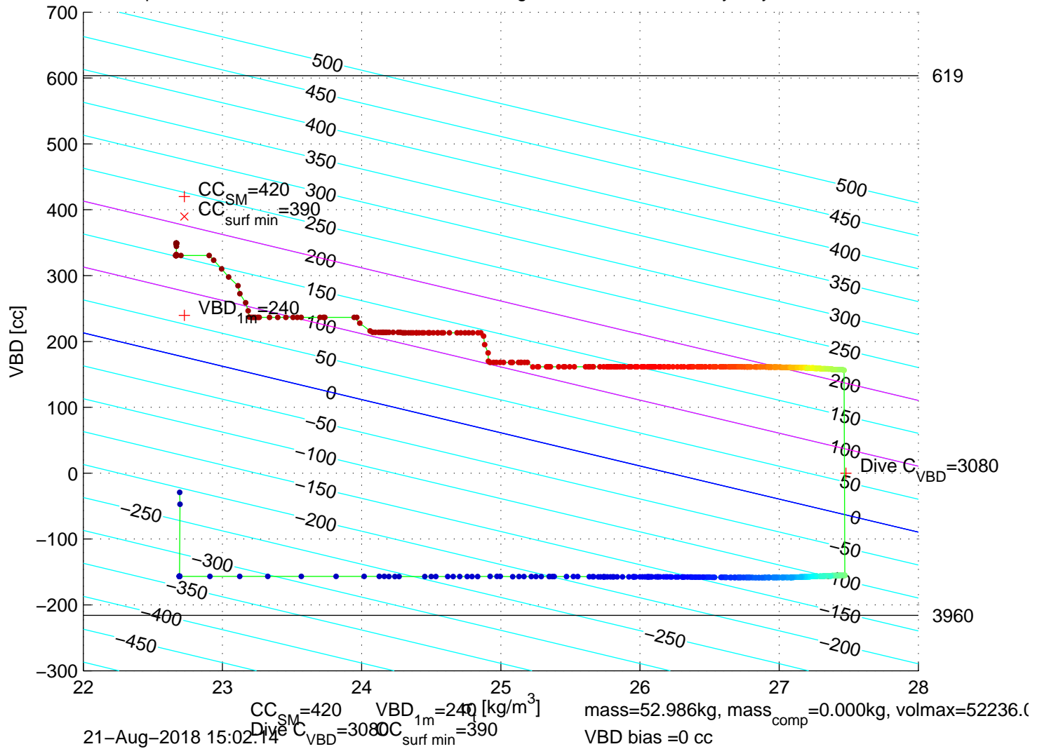
p6300118: SG630 Mission 8 Jul 2018 01–Aug–2018 04:20:15Z – buoyancy contoured
