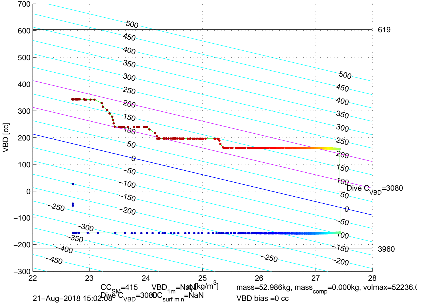
p6300110: SG630 Mission 8 Jul 2018 31-Jul-2018 00:40:35Z – buoyancy contoured
