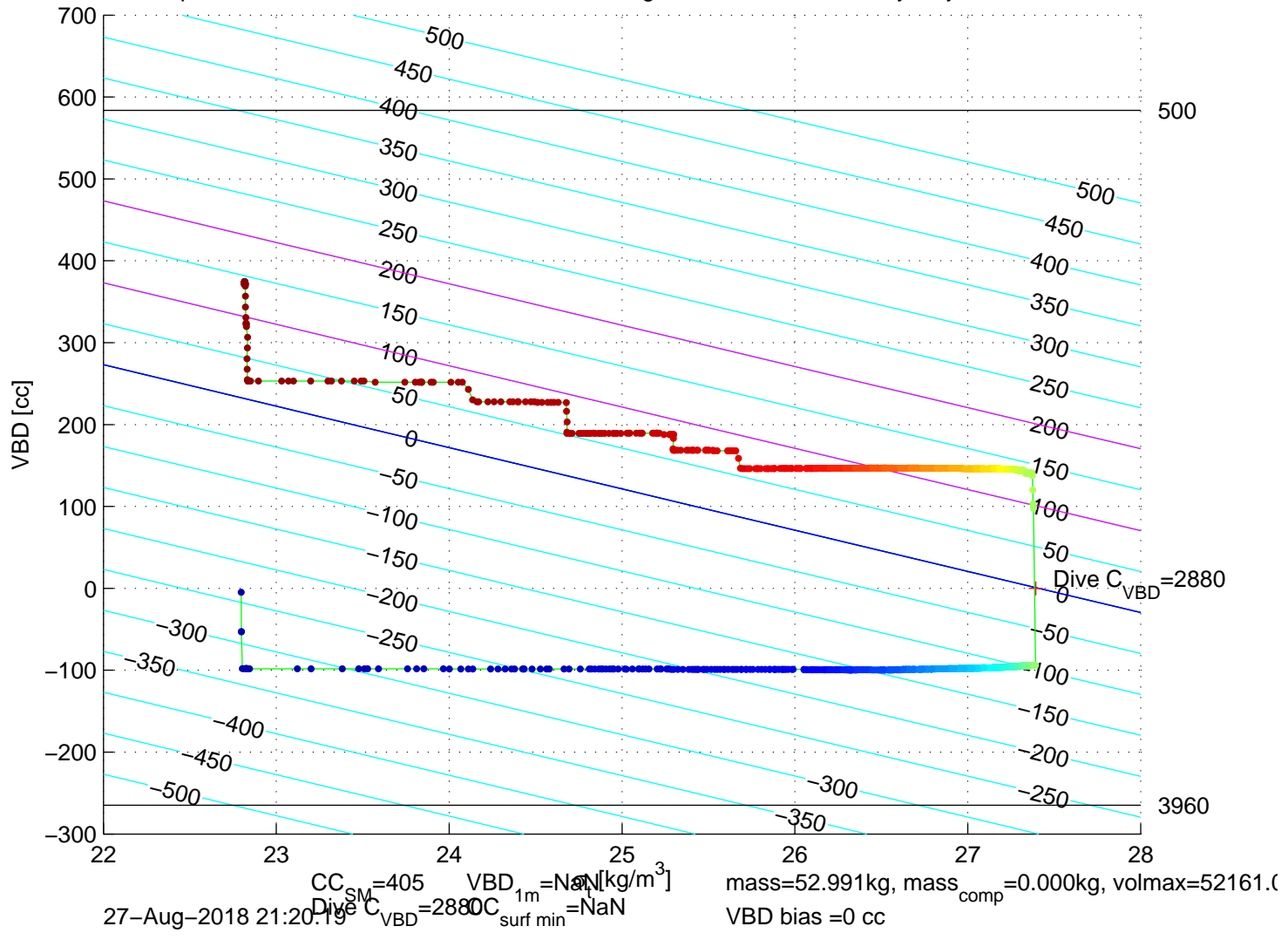
p6100225: SG610 Mission 8 Jul 2018 27-Aug-2018 20:53:40Z – buoyancy contoured
