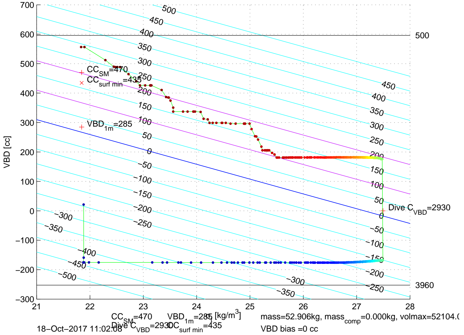
p6100654: SG610 Mission 7 Jul 2017 18–Oct–2017 10:24:42Z – buoyancy contoured
