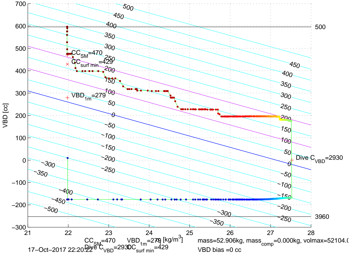
p6100651: SG610 Mission 7 Jul 2017 17-Oct-2017 21:43:36Z – buoyancy contoured
