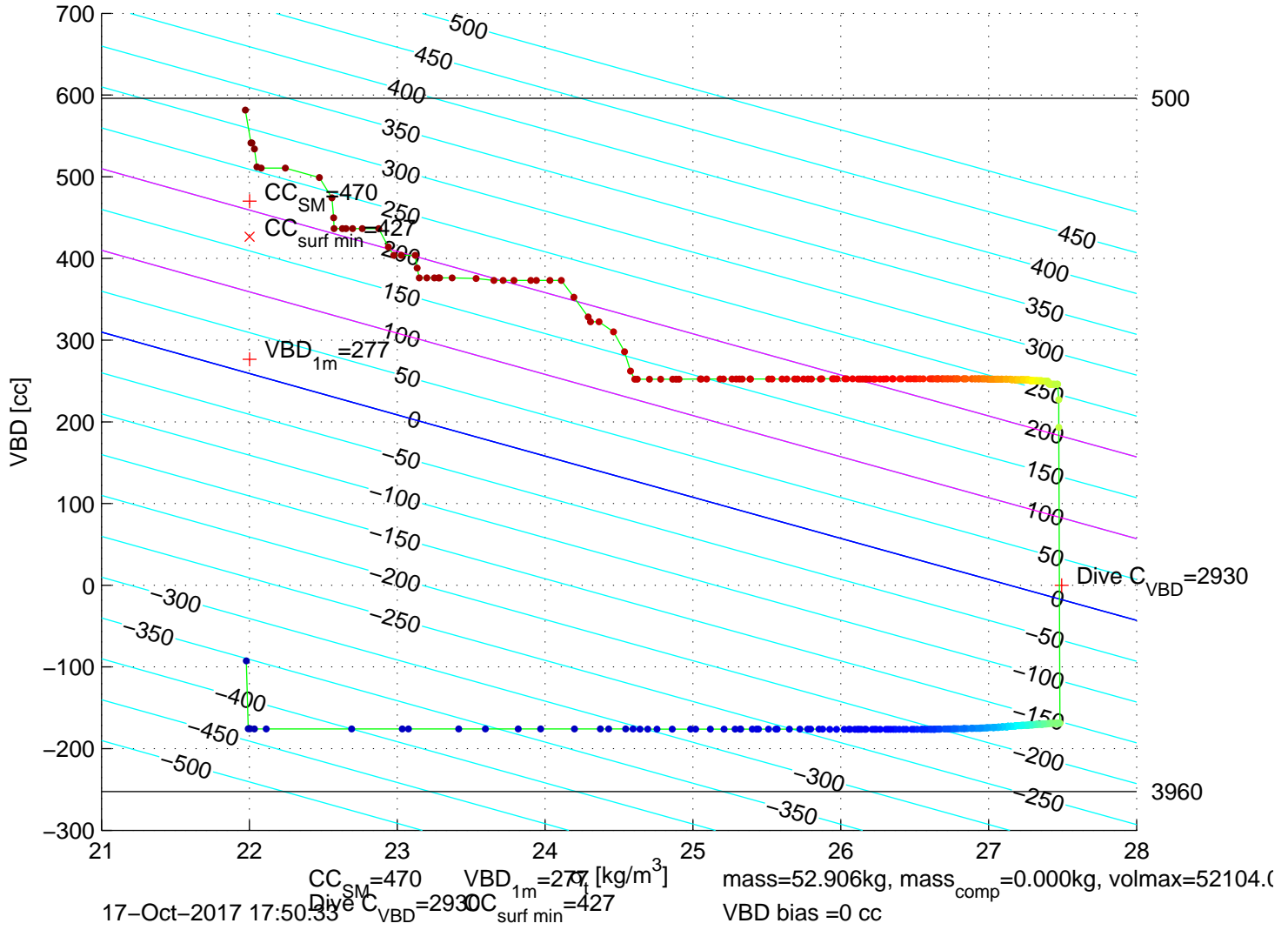
p6100650: SG610 Mission 7 Jul 2017 17-Oct-2017 17:34:13Z – buoyancy contoured
