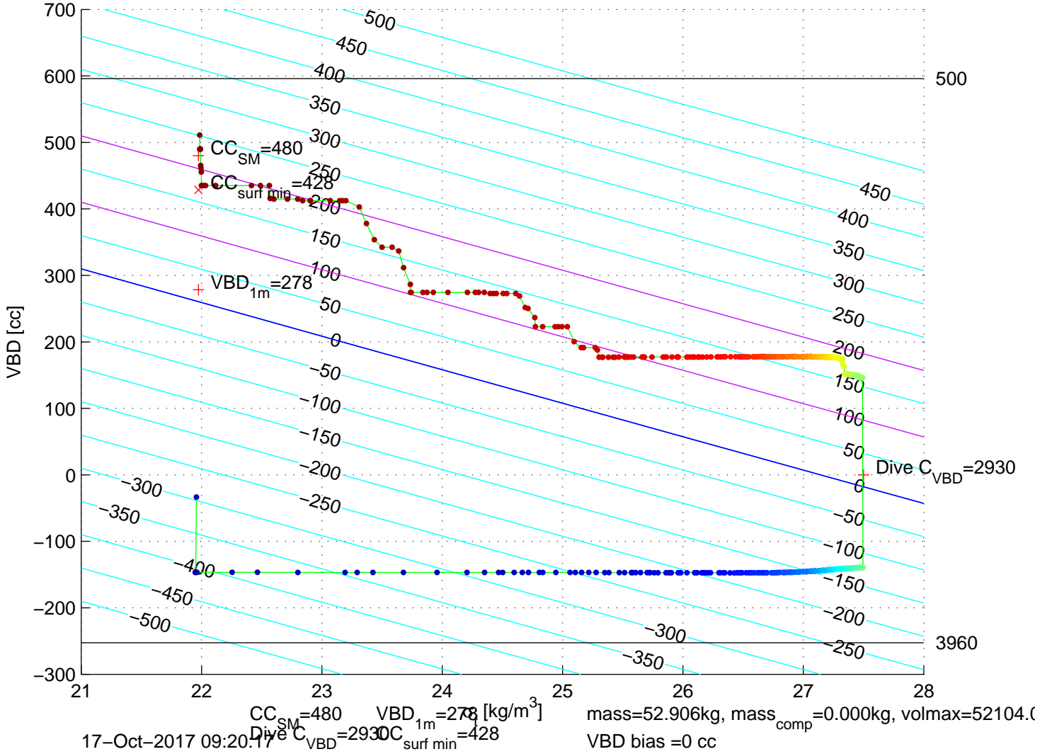
p6100648: SG610 Mission 7 Jul 2017 17-Oct-2017 08:50:10Z – buoyancy contoured
