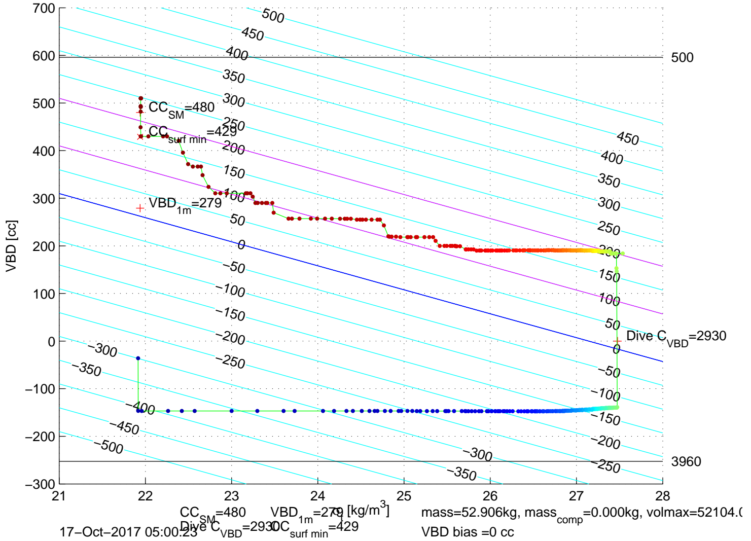
p6100647: SG610 Mission 7 Jul 2017 17-Oct-2017 04:32:49Z – buoyancy contoured
