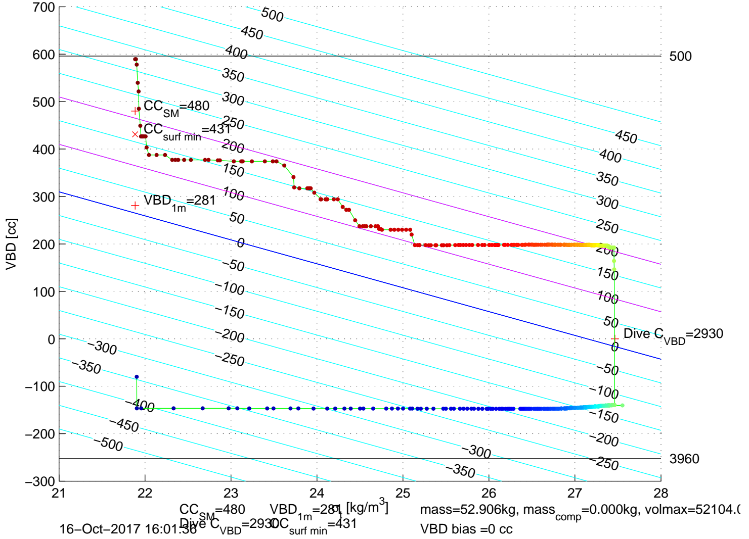
p6100644: SG610 Mission 7 Jul 2017 16–Oct–2017 15:33:53Z – buoyancy contoured
