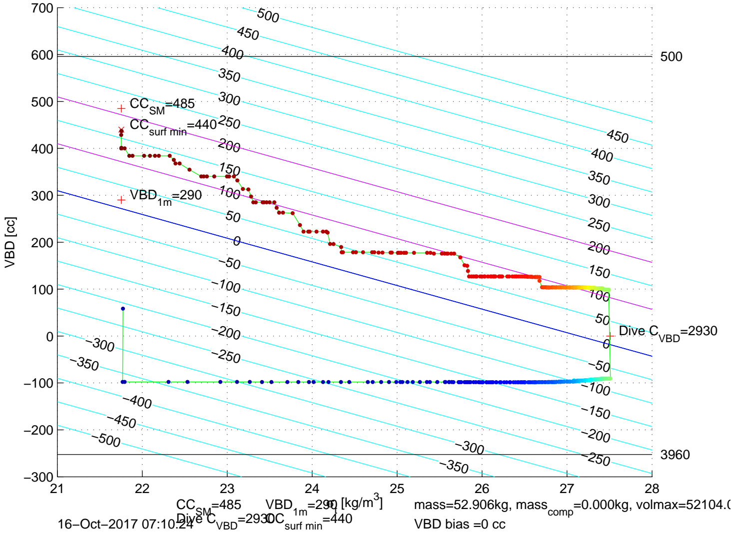
p6100642: SG610 Mission 7 Jul 2017 16–Oct–2017 06:21:00Z – buoyancy contoured
