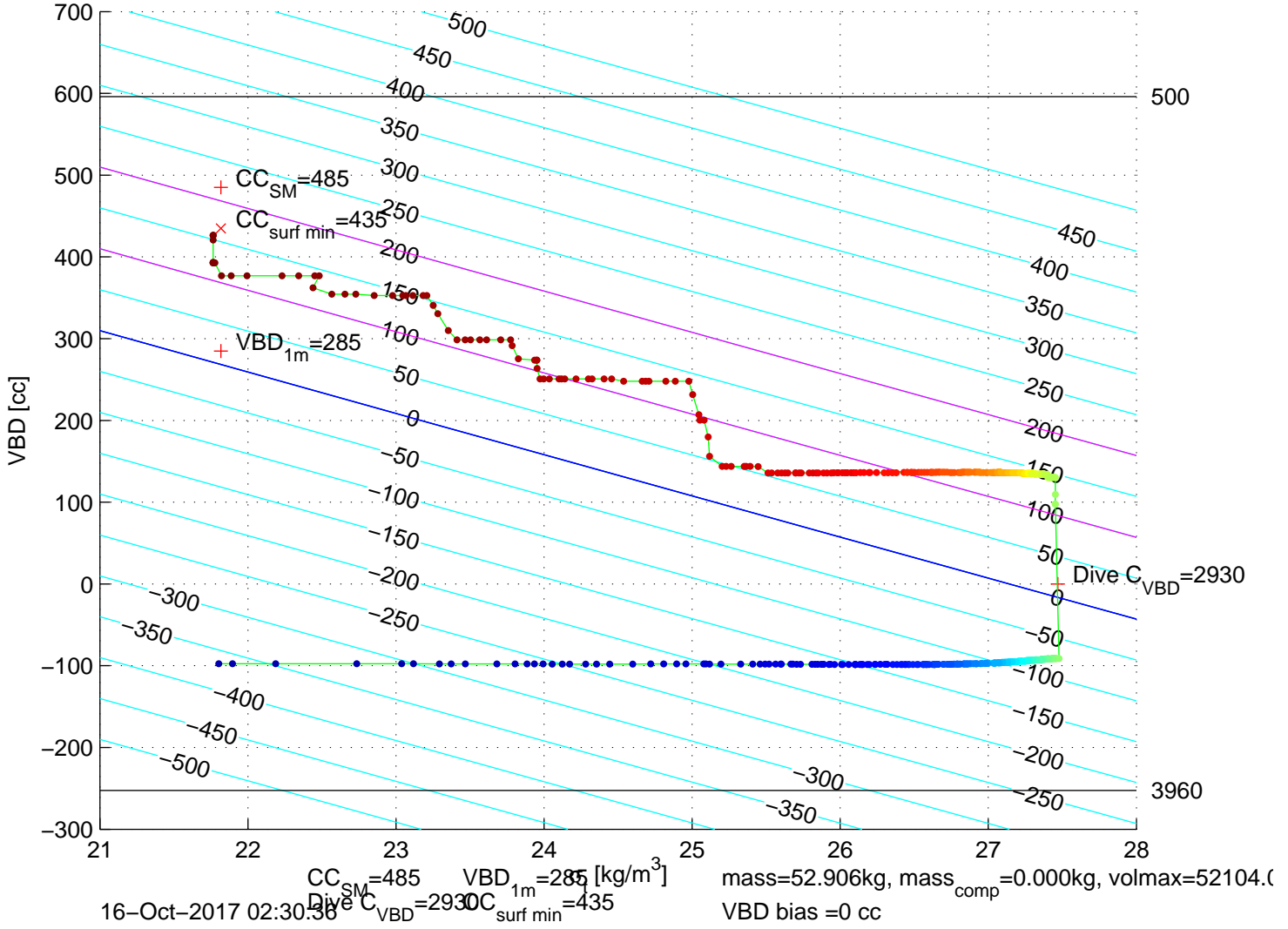
p6100641: SG610 Mission 7 Jul 2017 16–Oct–2017 01:53:34Z – buoyancy contoured
