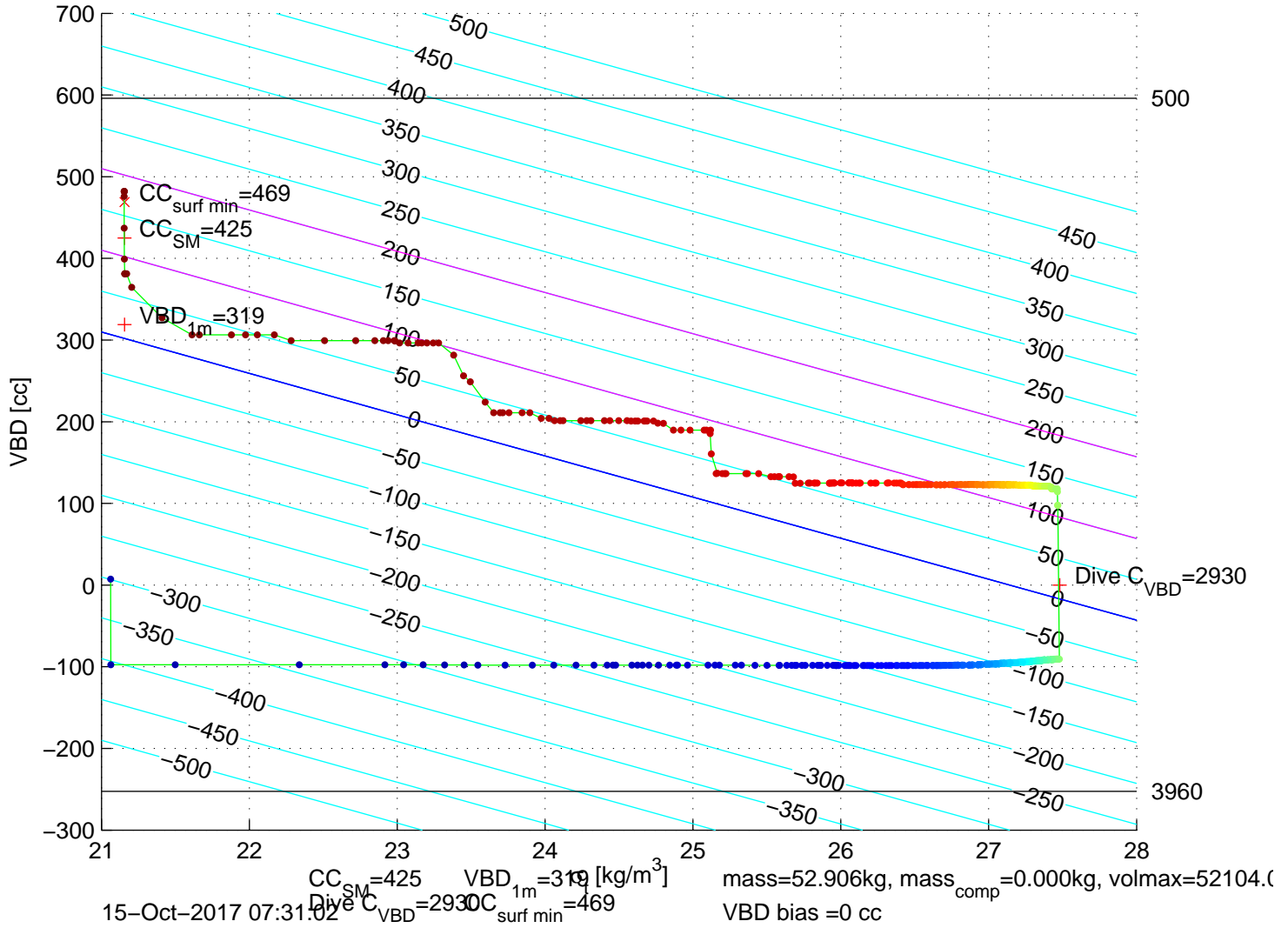
p6100637: SG610 Mission 7 Jul 2017 15-Oct-2017 06:43:28Z – buoyancy contoured
