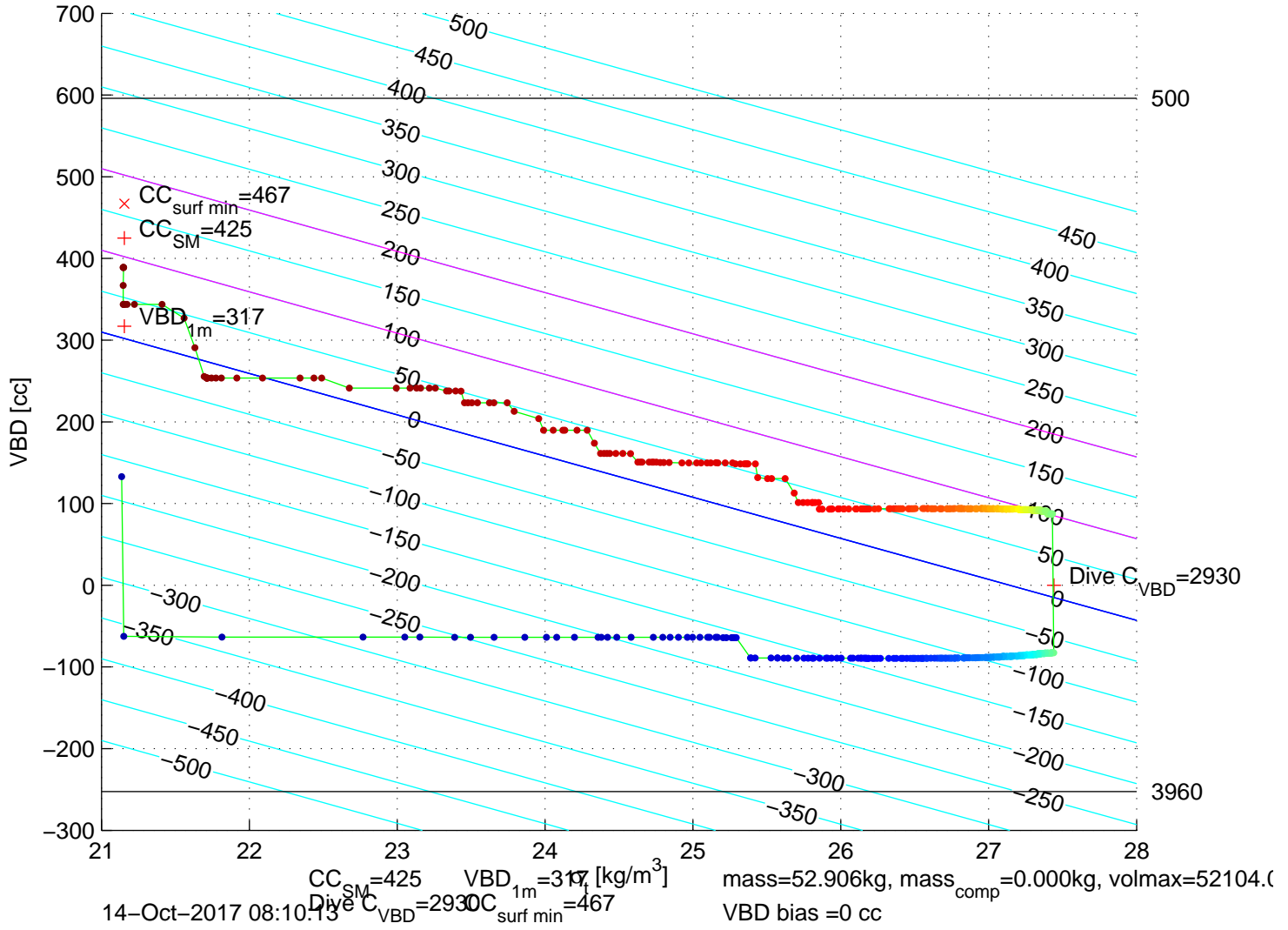
p6100632: SG610 Mission 7 Jul 2017 14-Oct-2017 07:38:36Z – buoyancy contoured
