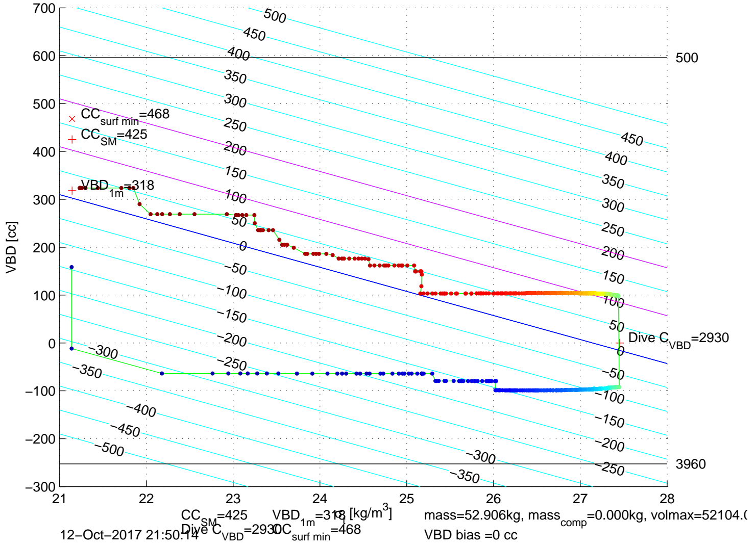
p6100624: SG610 Mission 7 Jul 2017 12–Oct–2017 21:24:25Z – buoyancy contoured
