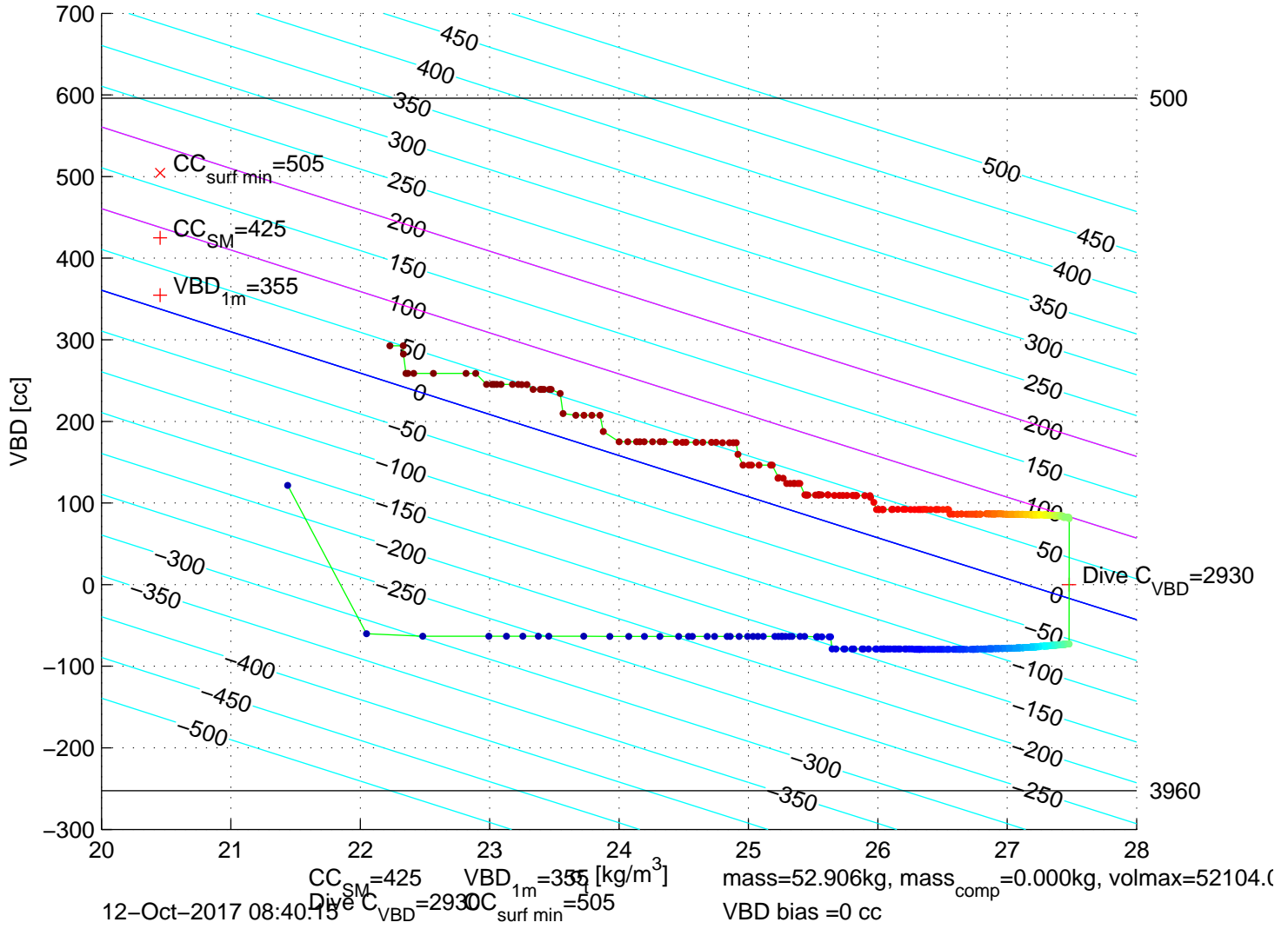
p6100621: SG610 Mission 7 Jul 2017 12–Oct–2017 07:56:02Z – buoyancy contoured
