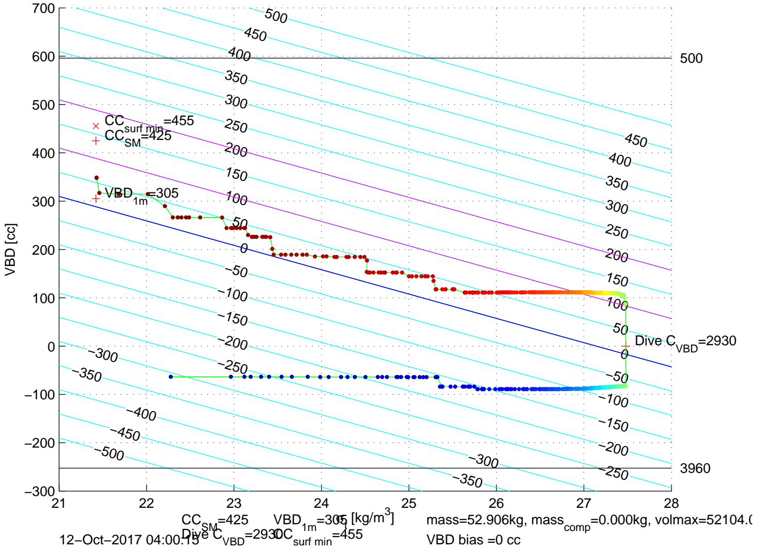
p6100620: SG610 Mission 7 Jul 2017 12-Oct-2017 03:43:46Z – buoyancy contoured
