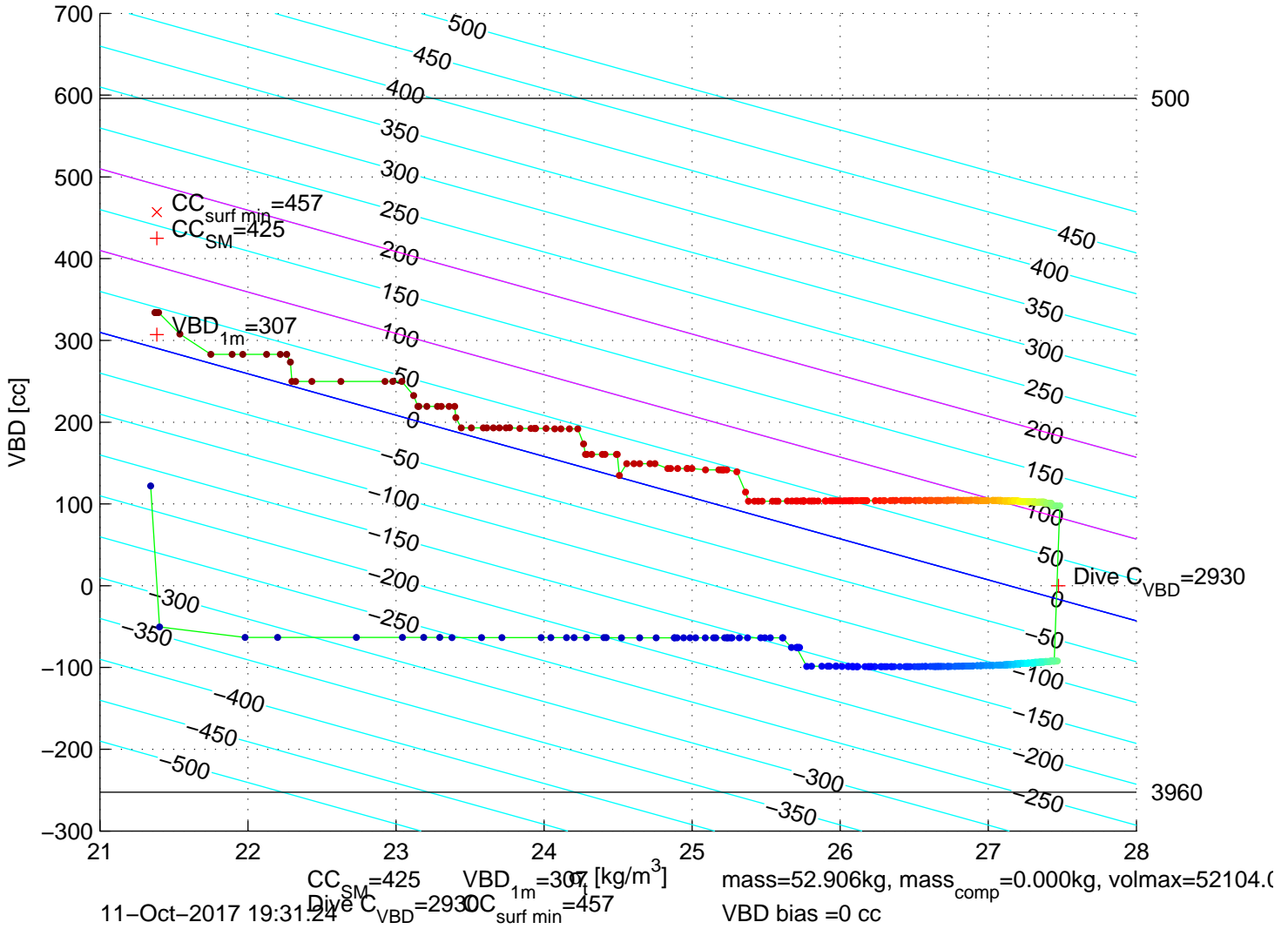
p6100618: SG610 Mission 7 Jul 2017 11–Oct–2017 19:05:01Z – buoyancy contoured
