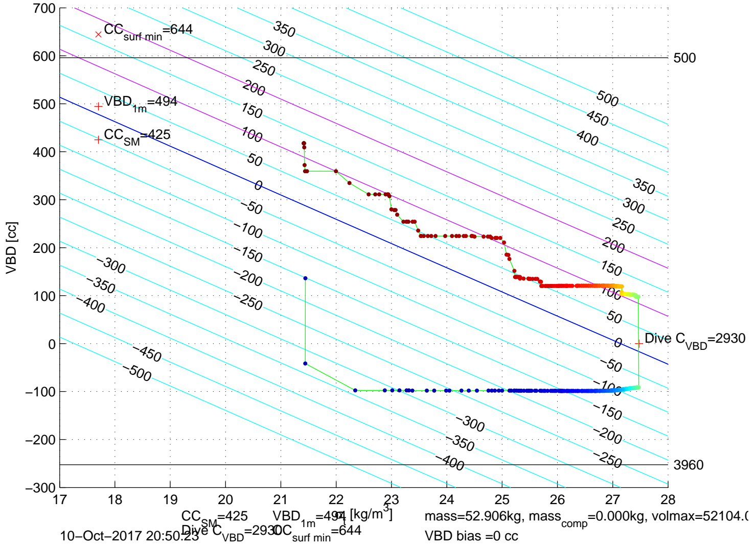
p6100613: SG610 Mission 7 Jul 2017 10–Oct–2017 20:05:29Z – buoyancy contoured
