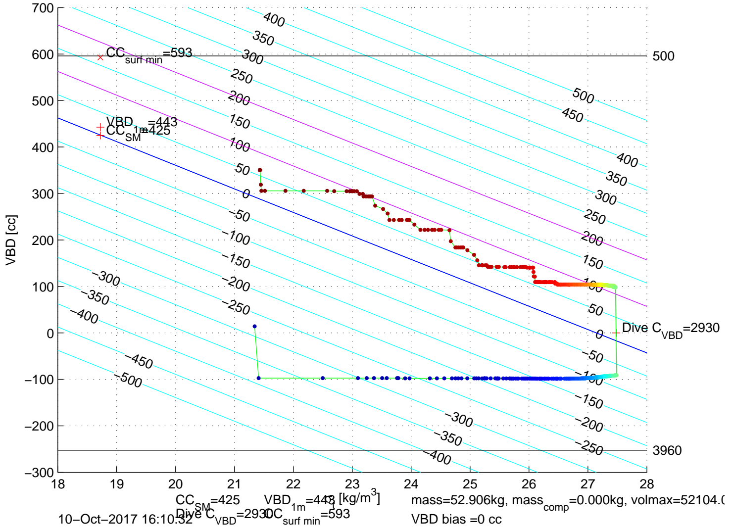
p6100612: SG610 Mission 7 Jul 2017 10–Oct–2017 15:16:46Z – buoyancy contoured
