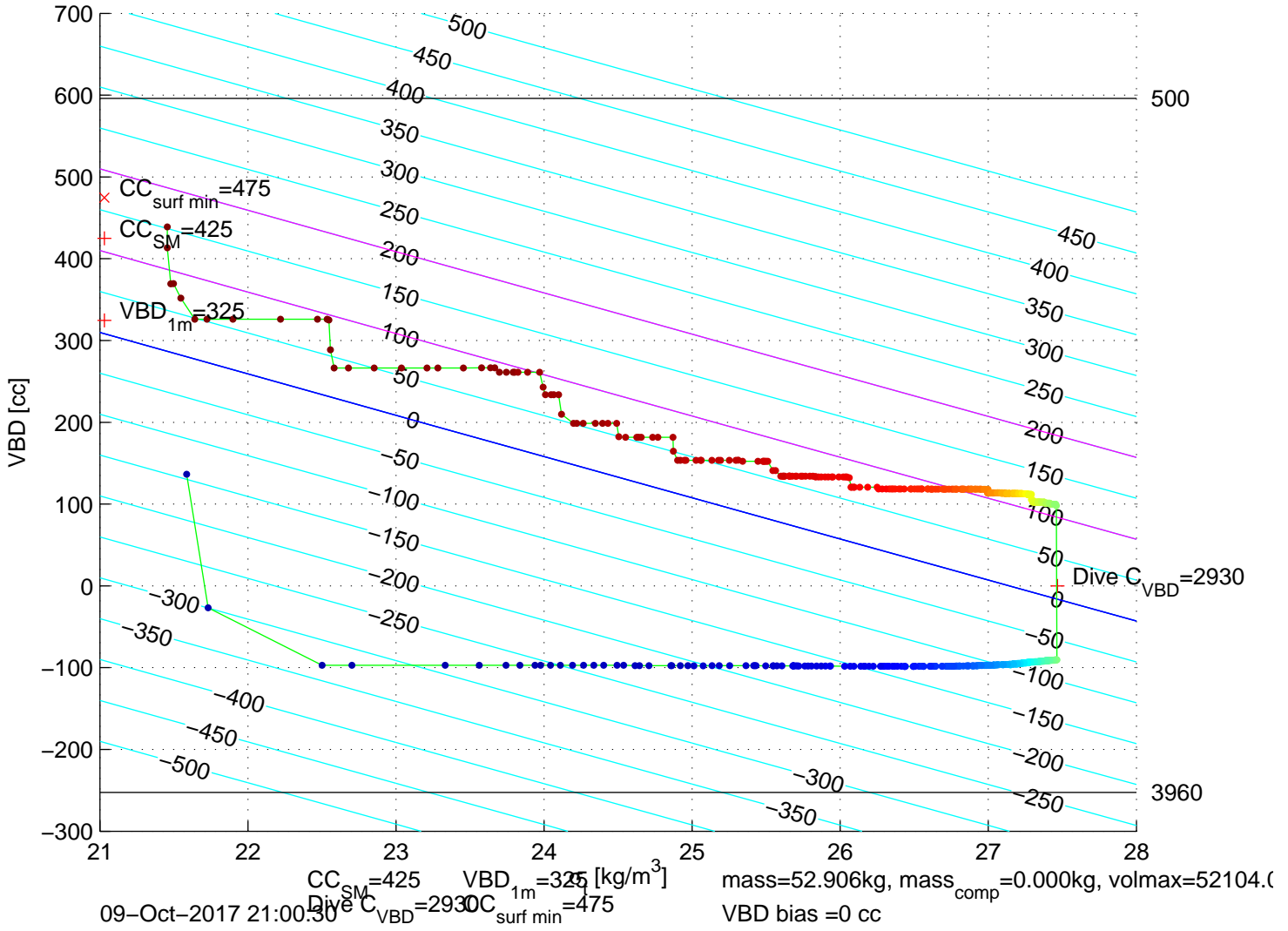
p6100608: SG610 Mission 7 Jul 2017 09–Oct–2017 20:14:10Z – buoyancy contoured
