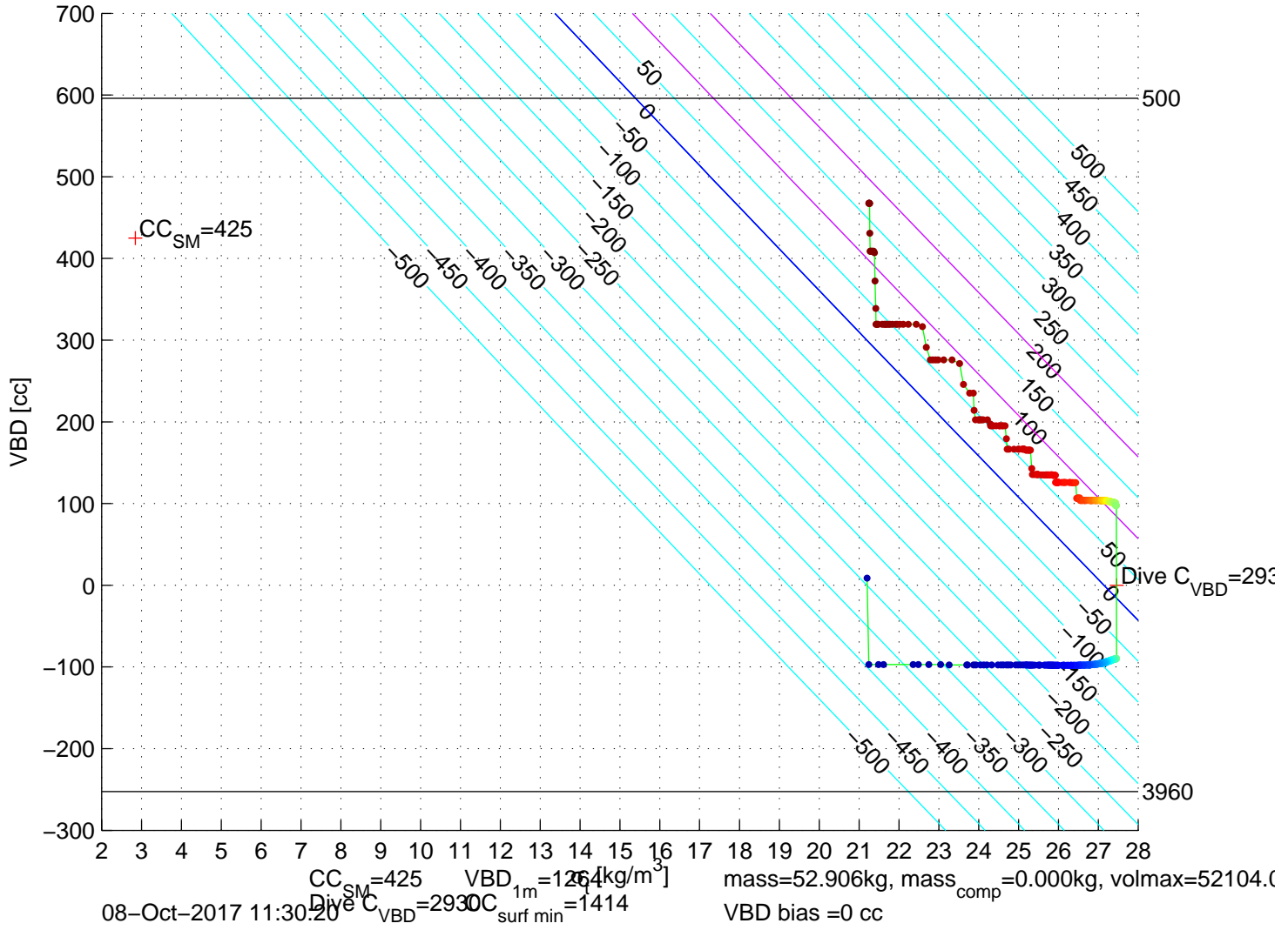
p6100601: SG610 Mission 7 Jul 2017 08–Oct–2017 10:21:11Z – buoyancy contoured
