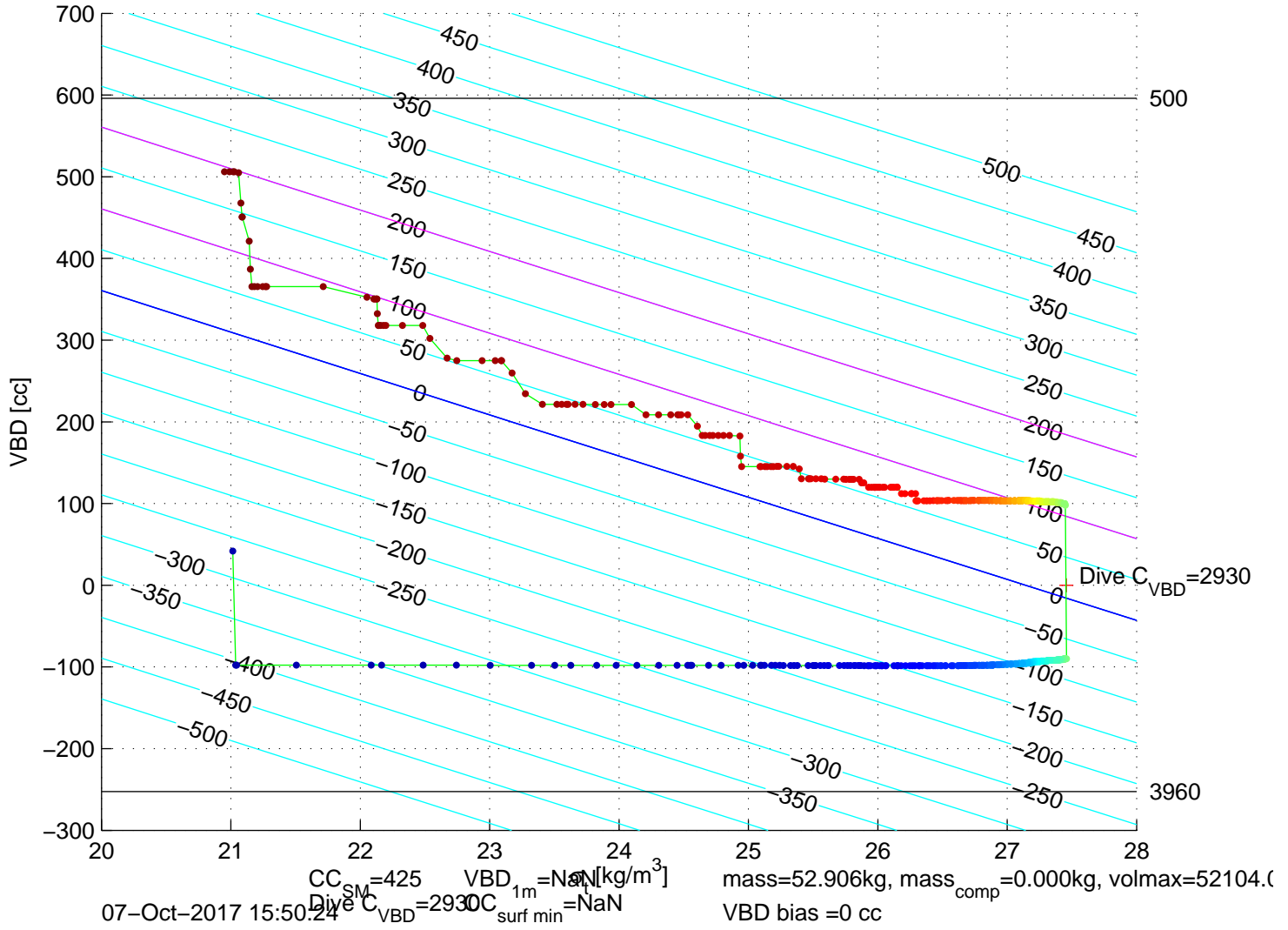
p6100597: SG610 Mission 7 Jul 2017 07–Oct–2017 14:52:12Z – buoyancy contoured
