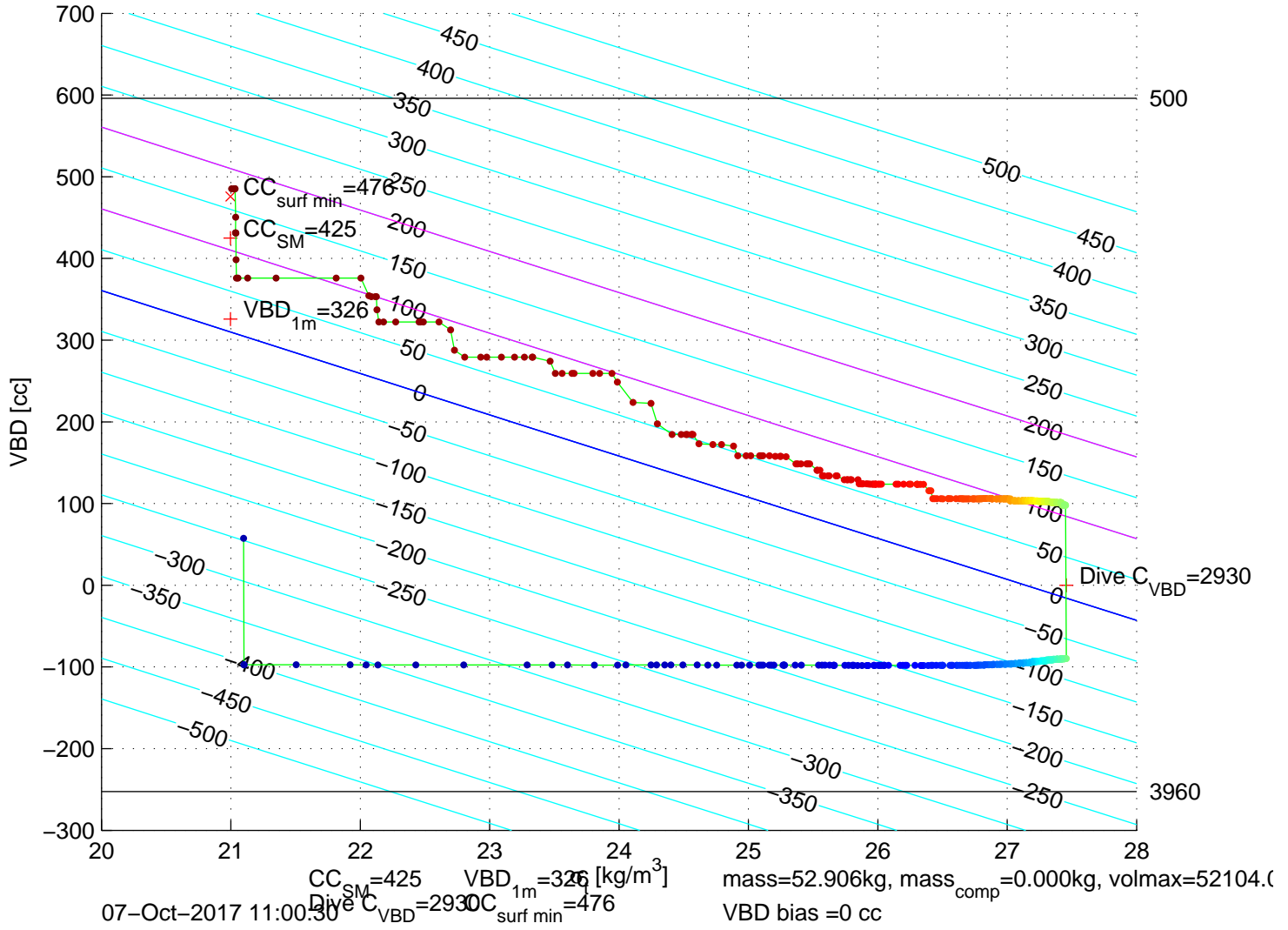
p6100596: SG610 Mission 7 Jul 2017 07–Oct–2017 10:03:51Z – buoyancy contoured
