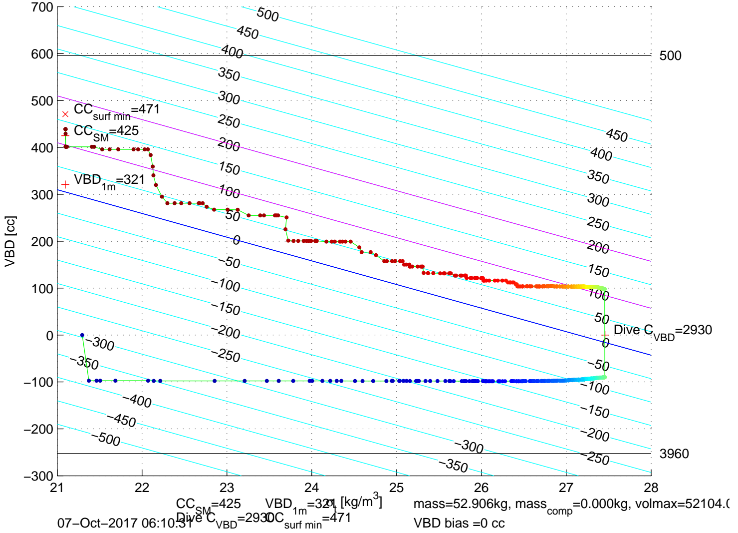
p6100595: SG610 Mission 7 Jul 2017 07–Oct–2017 05:11:46Z – buoyancy contoured
