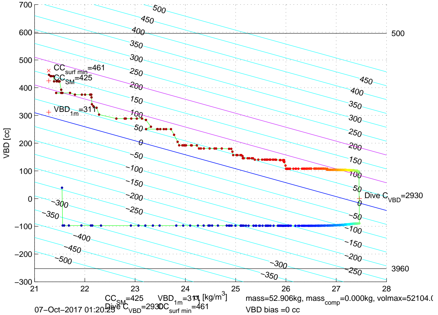
p6100594: SG610 Mission 7 Jul 2017 07–Oct–2017 00:22:54Z – buoyancy contoured
