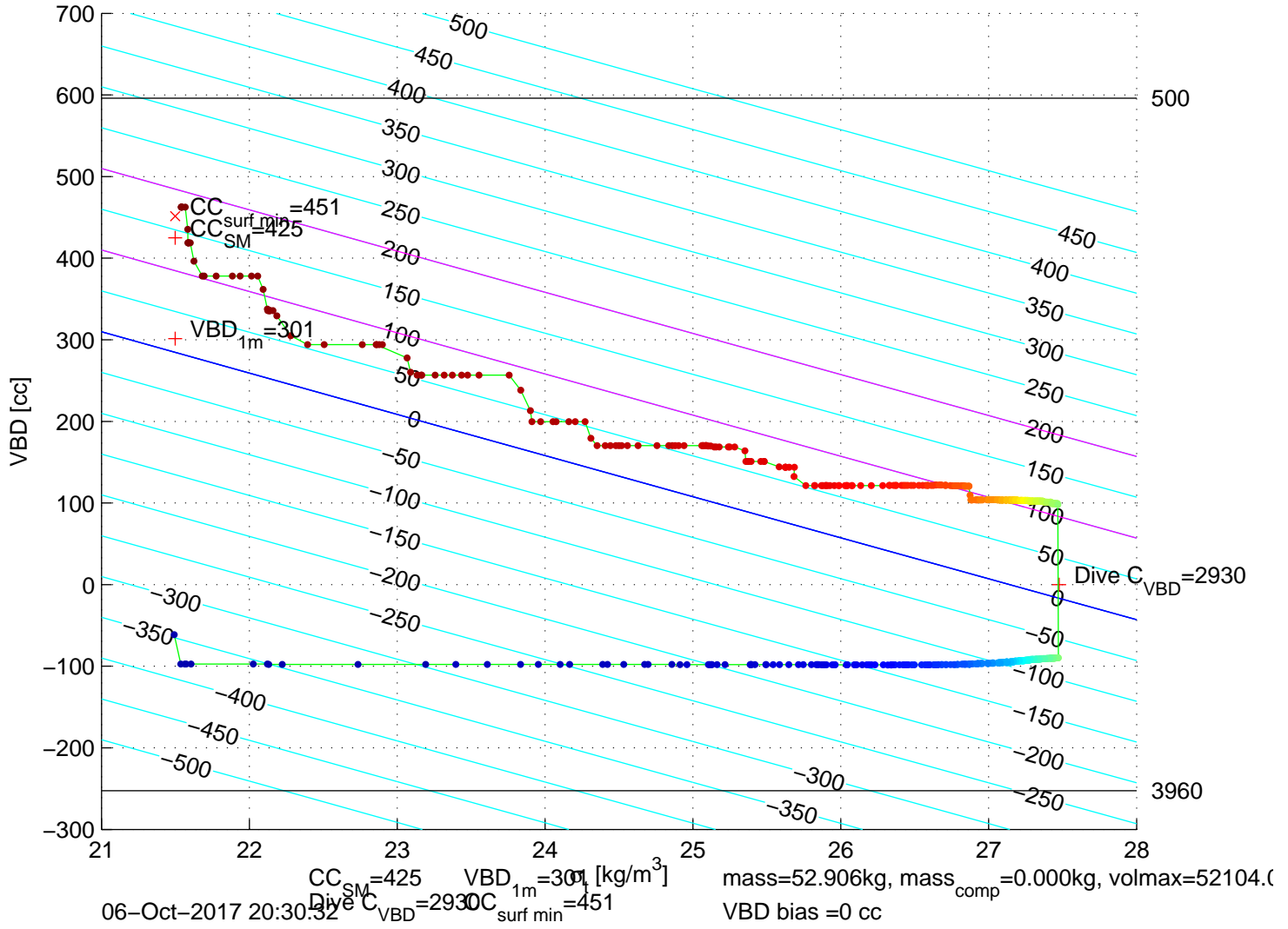
p6100593: SG610 Mission 7 Jul 2017 06–Oct–2017 19:31:56Z – buoyancy contoured
