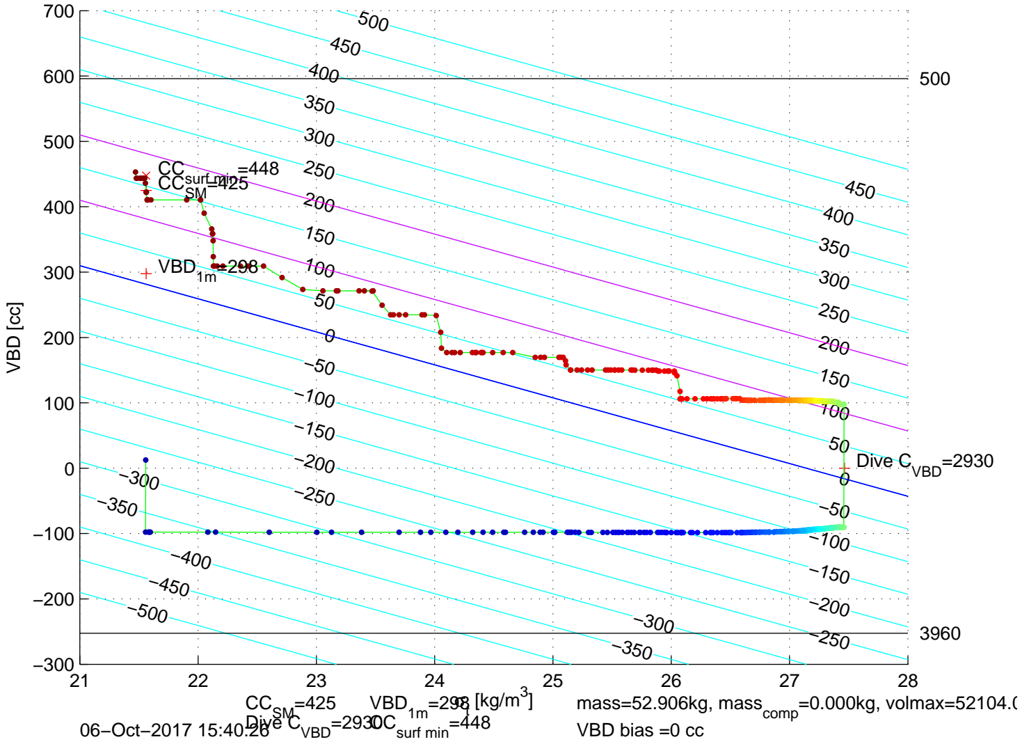
p6100592: SG610 Mission 7 Jul 2017 06–Oct–2017 14:39:33Z – buoyancy contoured
