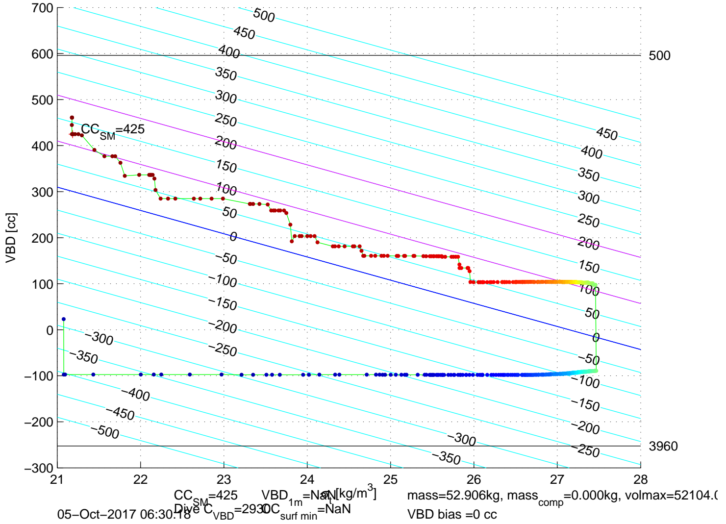
p6100585: SG610 Mission 7 Jul 2017 05–Oct–2017 05:32:20Z – buoyancy contoured
