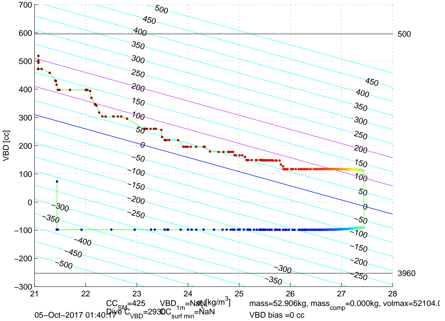
p6100584: SG610 Mission 7 Jul 2017 05-Oct-2017 00:52:01Z – buoyancy contoured
