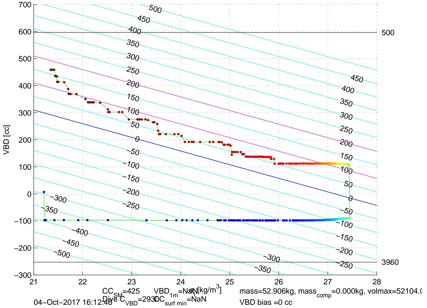
p6100582: SG610 Mission 7 Jul 2017 04–Oct–2017 15:18:45Z – buoyancy contoured
