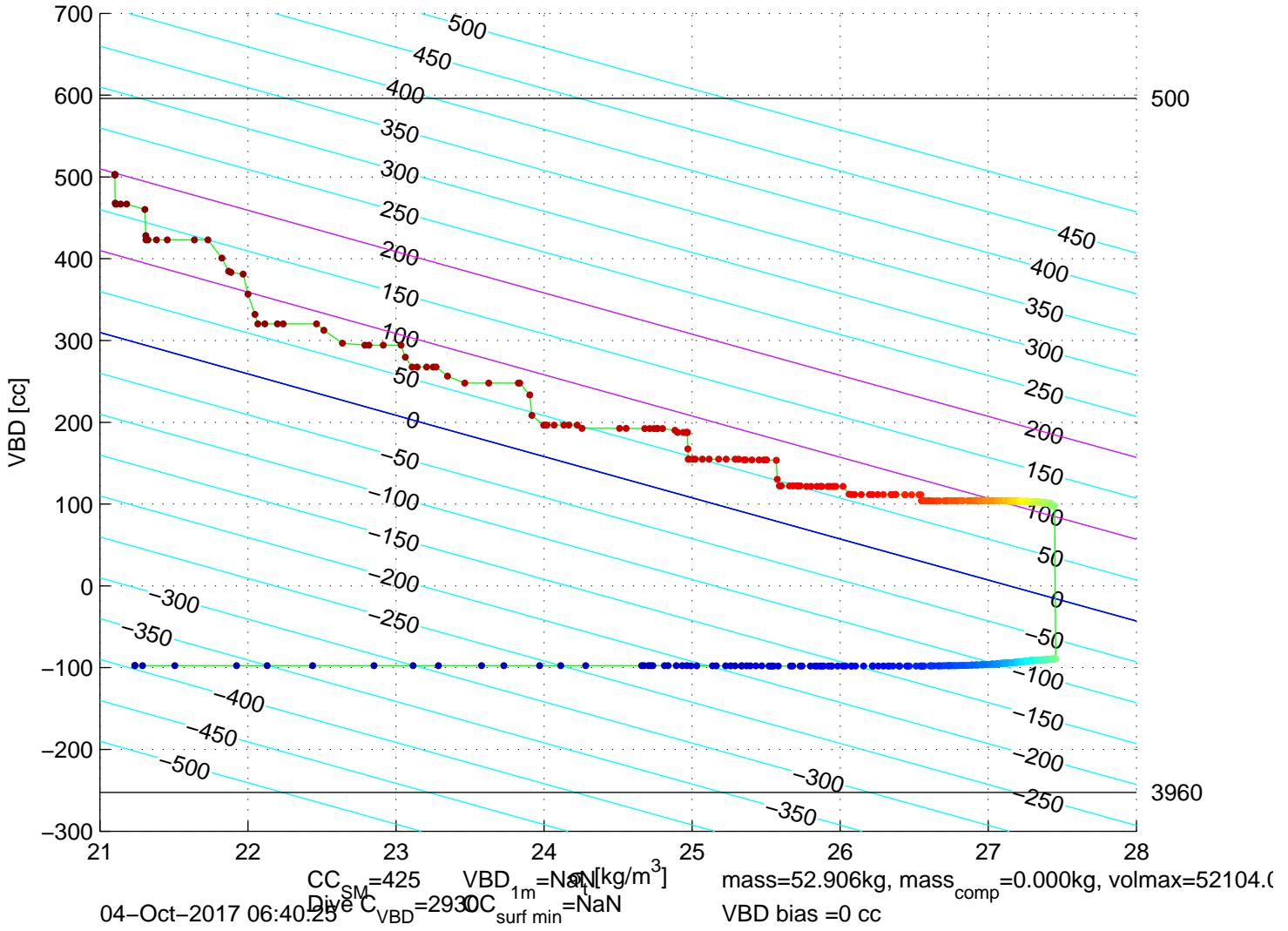
p6100580: SG610 Mission 7 Jul 2017 04–Oct–2017 05:38:08Z – buoyancy contoured
