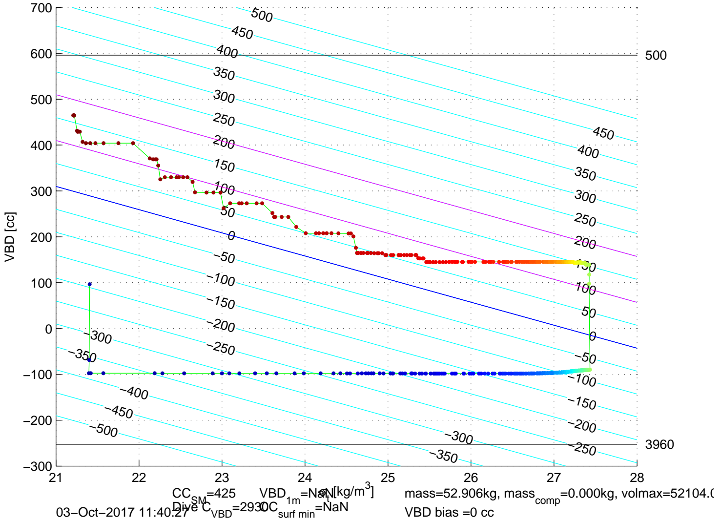
p6100576: SG610 Mission 7 Jul 2017 03-Oct-2017 11:09:26Z – buoyancy contoured
