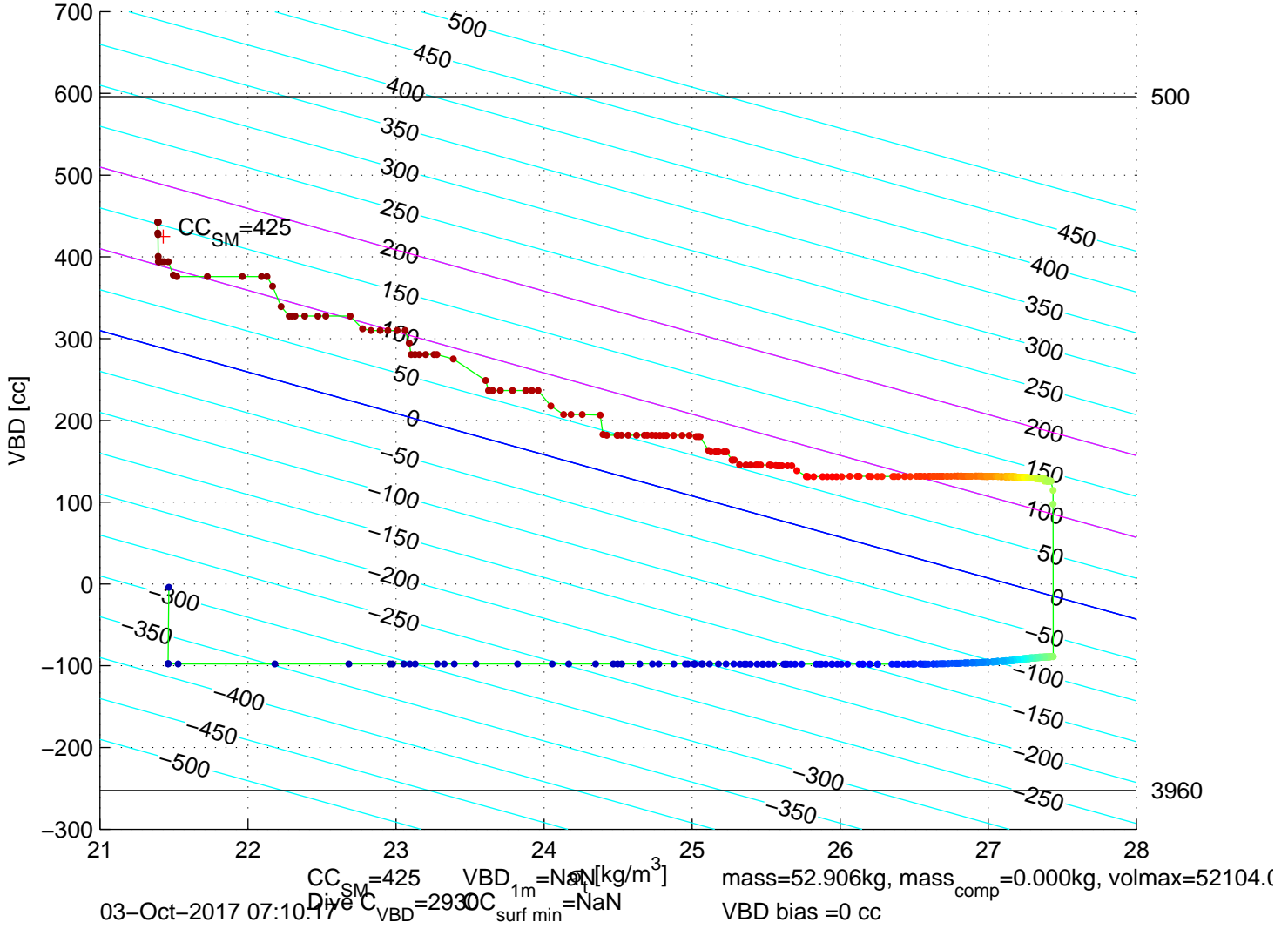
p6100575: SG610 Mission 7 Jul 2017 03–Oct–2017 06:32:38Z – buoyancy contoured
