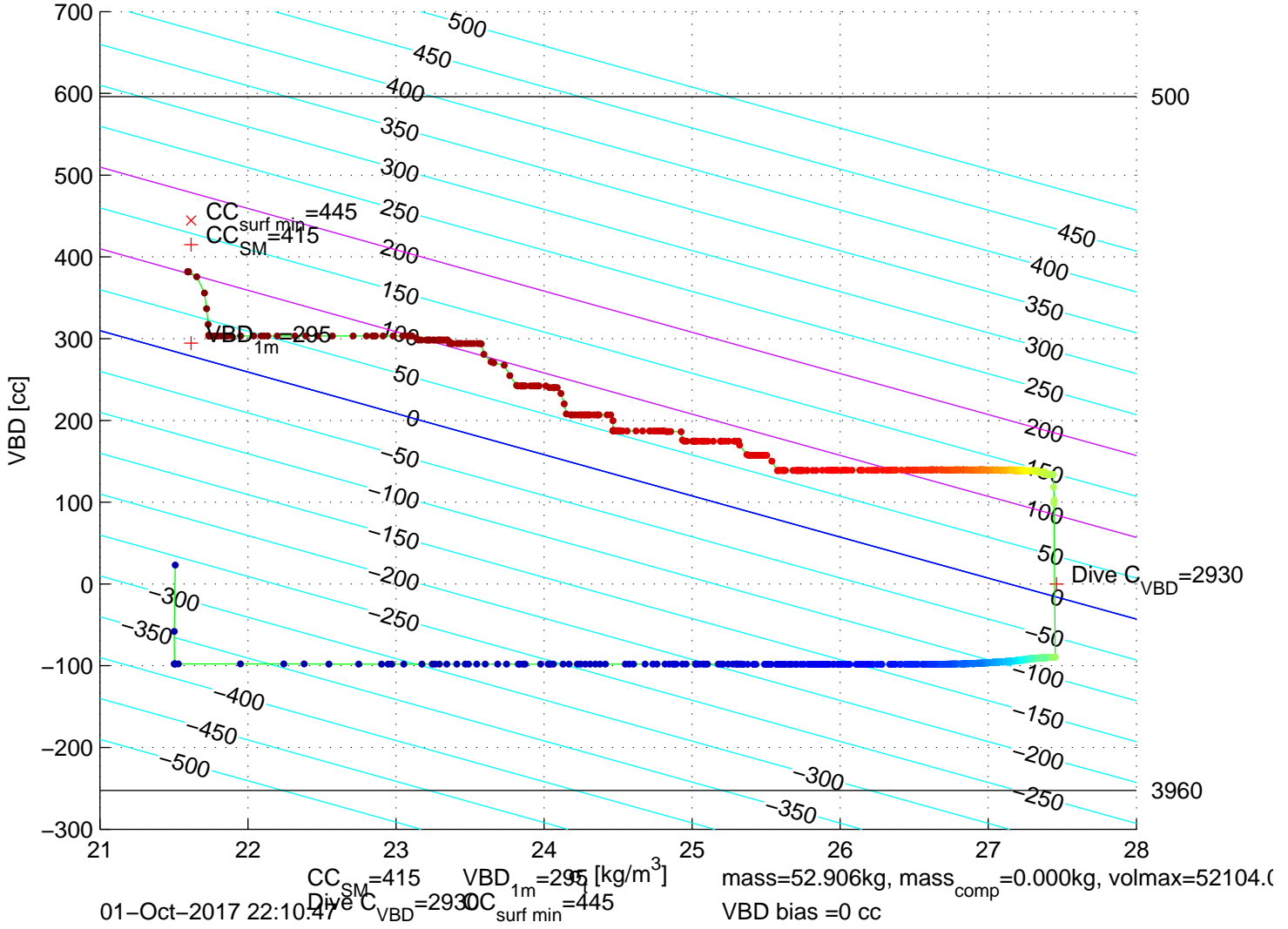
p6100568: SG610 Mission 7 Jul 2017 01–Oct–2017 21:14:31Z – buoyancy contoured
