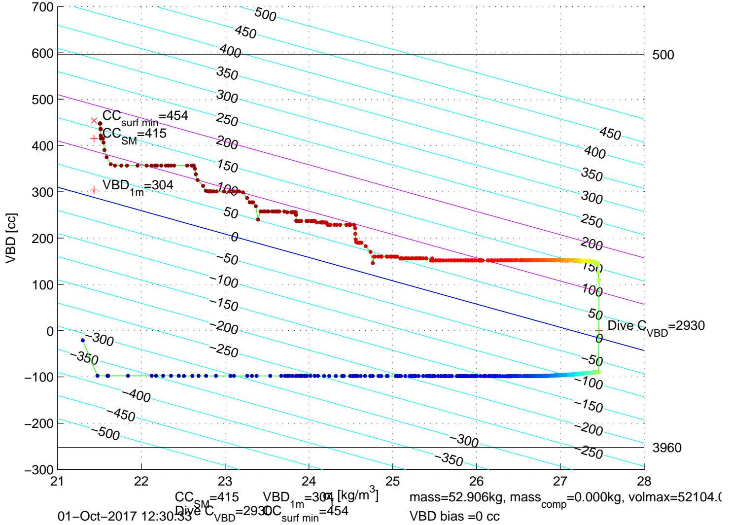
p6100566: SG610 Mission 7 Jul 2017 01–Oct–2017 11:48:05Z – buoyancy contoured
