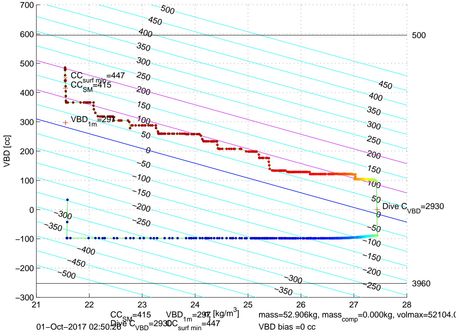
p6100564: SG610 Mission 7 Jul 2017 01–Oct–2017 01:48:45Z – buoyancy contoured
