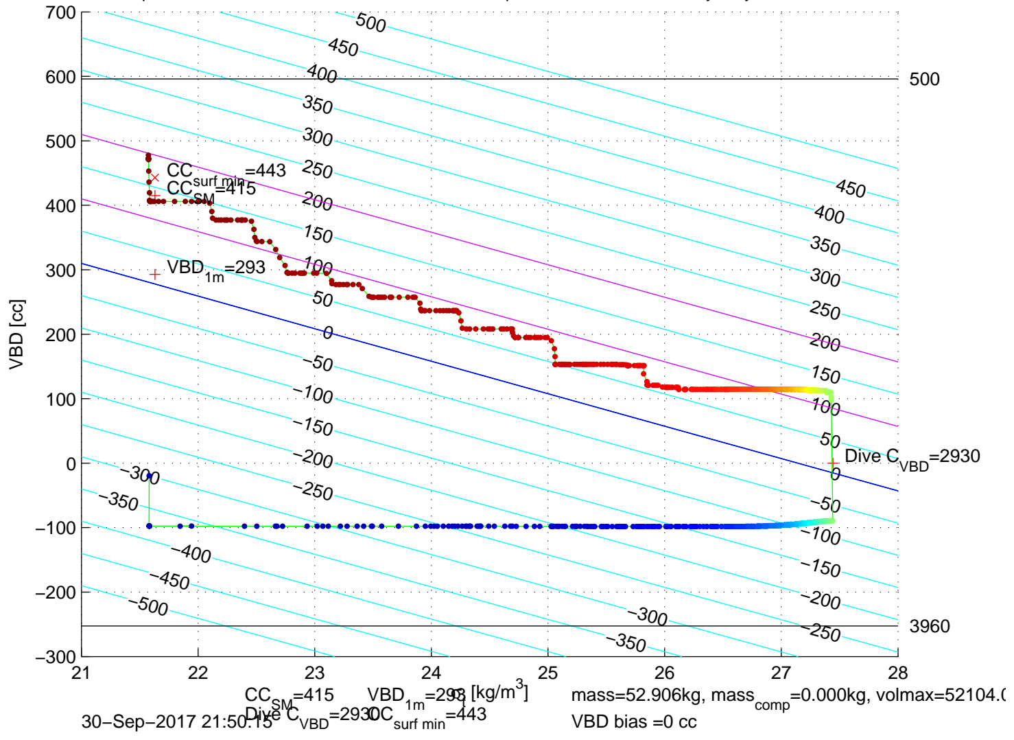
p6100563: SG610 Mission 7 Jul 2017 30-Sep-2017 20:50:46Z – buoyancy contoured
