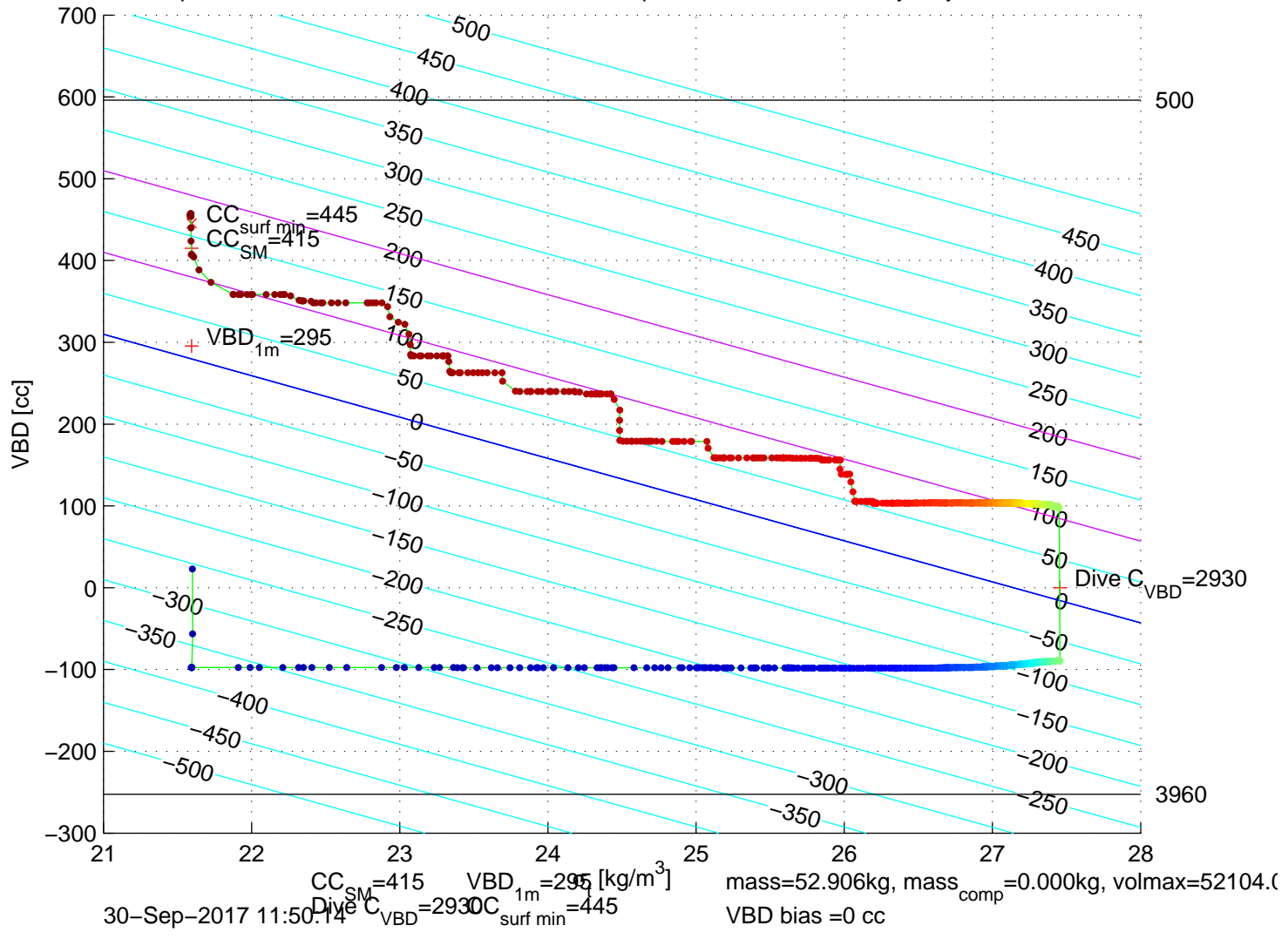
p6100561: SG610 Mission 7 Jul 2017 30-Sep-2017 10:48:21Z – buoyancy contoured
