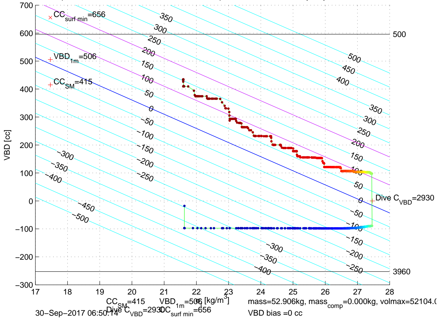
p6100560: SG610 Mission 7 Jul 2017 30-Sep-2017 05:47:54Z – buoyancy contoured
