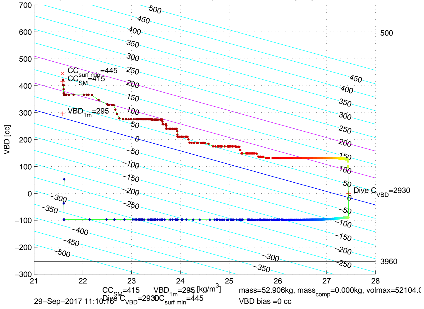
p6100556: SG610 Mission 7 Jul 2017 29-Sep-2017 10:24:39Z – buoyancy contoured
