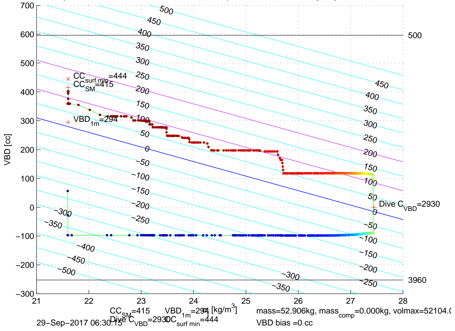
p6100555: SG610 Mission 7 Jul 2017 29-Sep-2017 05:32:38Z – buoyancy contoured
