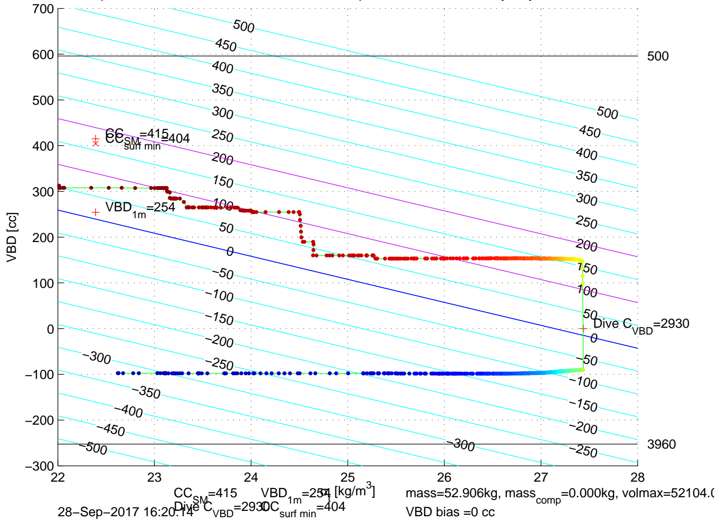
p6100552: SG610 Mission 7 Jul 2017 28-Sep-2017 15:38:46Z – buoyancy contoured
