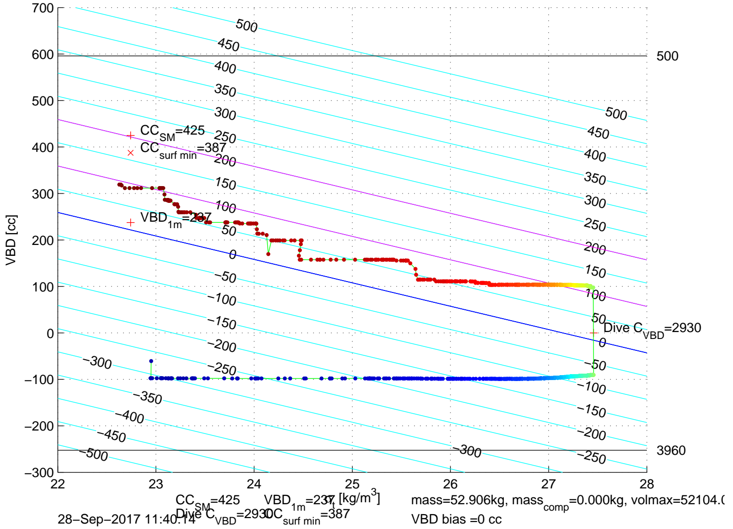
p6100551: SG610 Mission 7 Jul 2017 28-Sep-2017 10:40:29Z – buoyancy contoured
