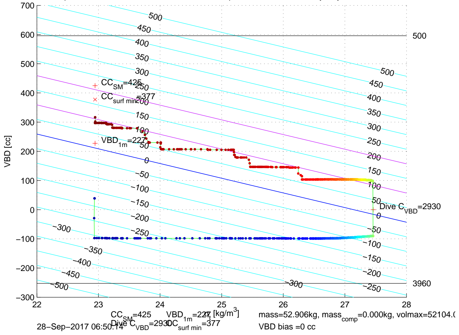
p6100550: SG610 Mission 7 Jul 2017 28-Sep-2017 05:45:03Z – buoyancy contoured
