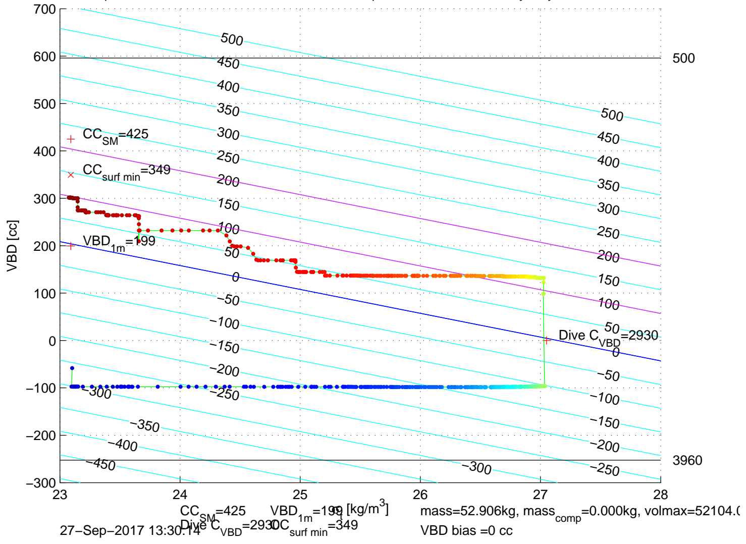
p6100546: SG610 Mission 7 Jul 2017 27-Sep-2017 14:48:21Z – buoyancy contoured
