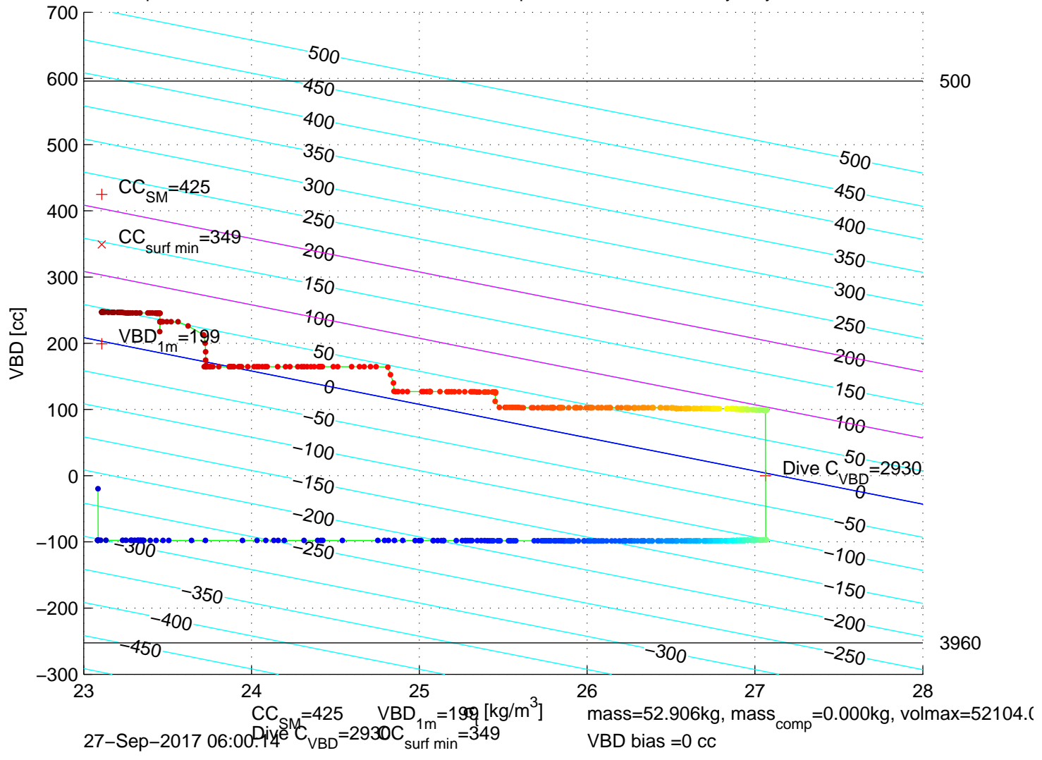
p6100543: SG610 Mission 7 Jul 2017 27-Sep-2017 07:22:14Z – buoyancy contoured
